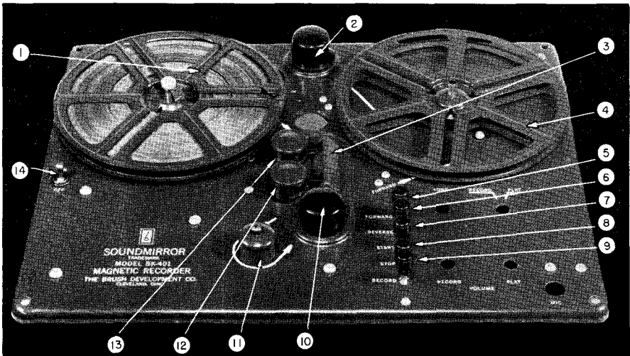
Fig. 12-16. Top view of Brush "Soundmirror" tape recorder. Keyed parts are; (1) Supply reel; (2) Reverse limit switch; (3) Brake shoe for head; (4) Takeup reel; (5) Forward push-bottom; (6) Reverse push-button; (7) Start push-button; (8) Stop push-button; (9) Record push-button; (10) Forward limit switch; (11) Drive capstan; (12) Record-reproduce head; (13) Erase head, and (14) On-off toggle switch.
