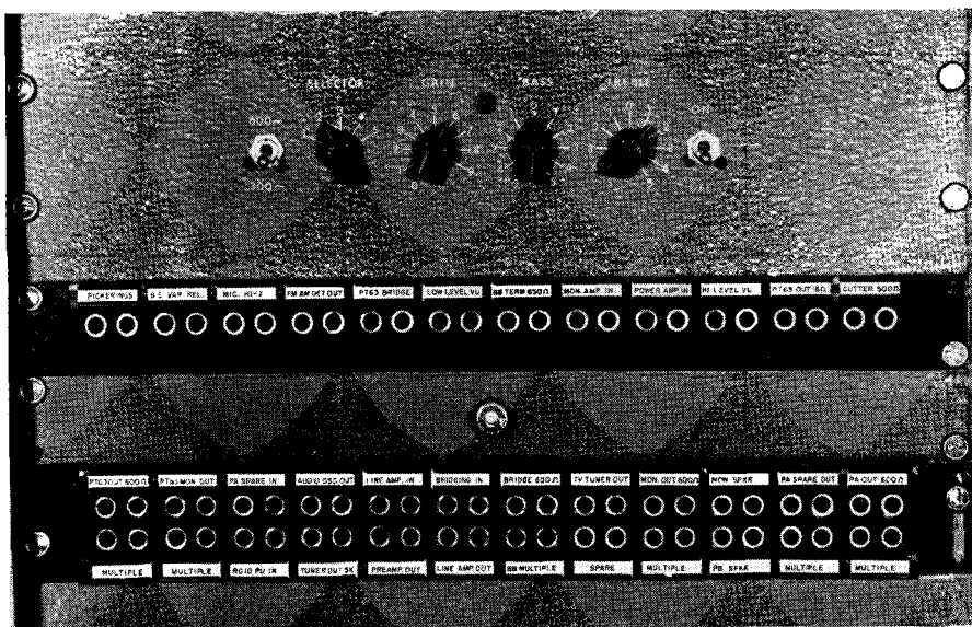
Fig. 26-3. All program circuits terminate in this jack field mounted below the AE-2 preamp-equalizer. (Courtesy RADIO & TELEVISION NEWS)
