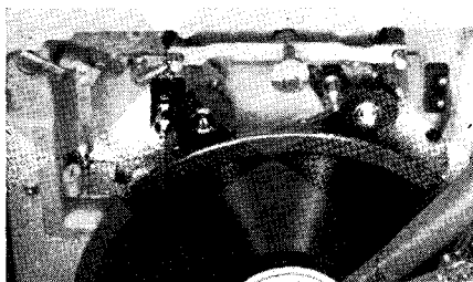
Fig. 5-18. The brake shoe moves away from turntable rim and the idlers are now in contact with the drive wheel in the "on" position.
