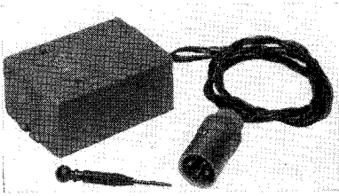
Fig. 5-8. The RCA MI-11850-C Professional recording head.
