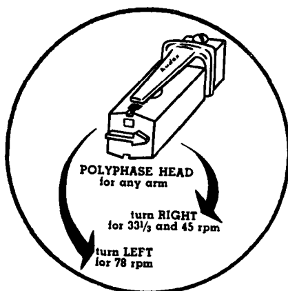
Fig. 9-30. (A) The Audax Polyphase reproducer ready for mounting within tone arm. (B) Showing how either stylus for standard or for LP is selected by simply rotating cartridge.
