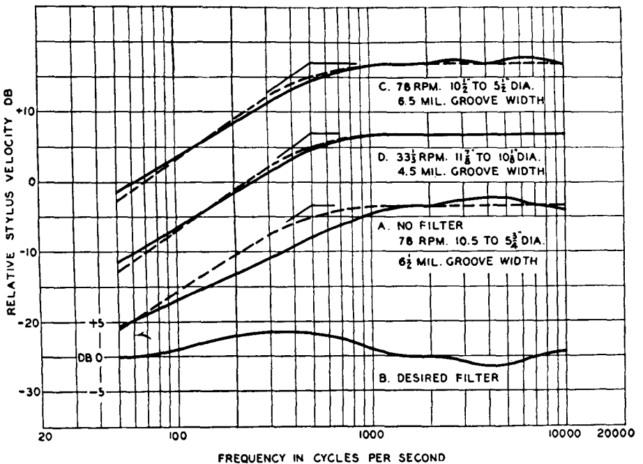
Fig. 5-32. Characteristics of another cutter without and with filter adjusted for proper crossover and smooth response.
