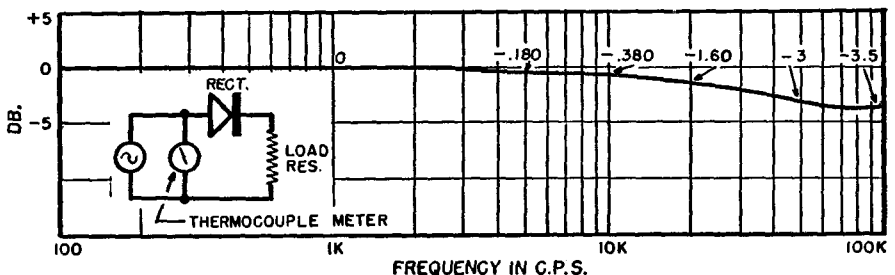
Fig. 8-7. Frequency response of a conventional copper-oxide instrument rectifier.
