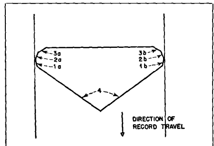
Fig. 7-18. Cross-section of an Anti-Noise Modulation Stylus provided with three burnishing facets, each 0.0001" wide. The leading facet (3a-3b) is polished at an angle of 60°; the middle facet (2a-2b) at 25°; the trailing facet (1a-1b) at minus 10°. The clearance faces (4) are polished at 35° to provide additional clearance in 45° groove slopes. (Courtesy, F. L. Capps)
