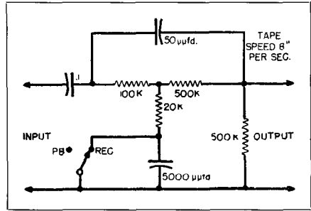
Fig. 12-9. Equalizer circuit for magnetic tape recording.
