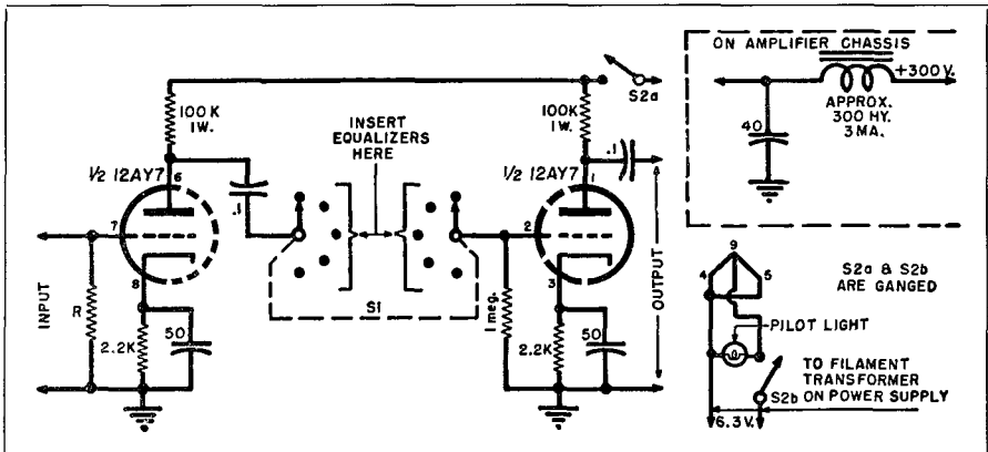
Fig. 20-5. Circuit diagram of preamplifier. Equalizers connect to Switch S1.
