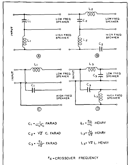
Fig. 16-3. Four types of constant-resistance networks and associated formulas for computing values. See note in text on A and B.
