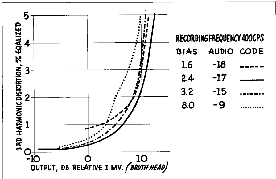
Fig. 11-21. Distortion as a Function of Output for Various Bias Currents. 'Scotch' Sound Recording Tape No. 111.
