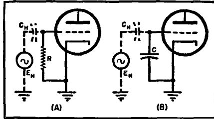
Fig. 28-32. (A) Capacitive hum pickup. (B) Capacitive hum pickup in crystal microphone or in phonograph input circuits.
