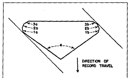
Fig. 7-19. Stylus cross-section of Fig. 7-18 in a groove slope of 45°. Here facet 1a (polished at minus 10°) burnishes the adjacent groove wall at 35°. On the opposite side leading facet 3b (polished at 60°) burnishes its adjacent groove wall at 15°. (Courtesy, F. L. Capps)
