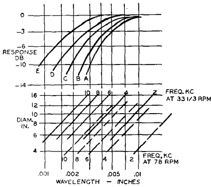
Fig. 7-28. Playback response vs. wavelength of recorded waves. The lower family of curves relates the wavelength to the frequencies and diameter of records turning at 78 and 33 1/3 rpm.
