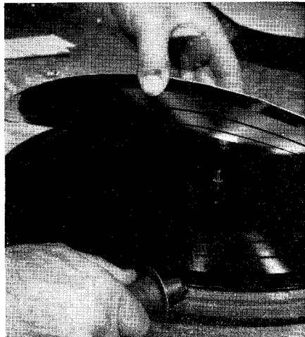
Fig. 27-4. Stripping the metal "master" from the "master" recording.
