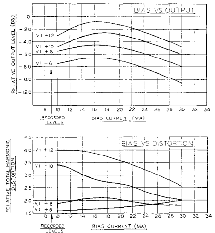
Fig. 13-9. Magnetic recording characteristics.
