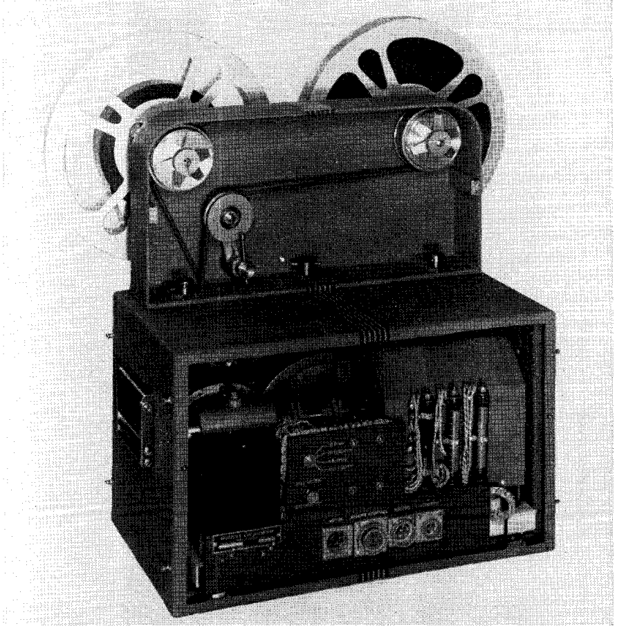
Fig. 13-4. Rear view of the RA-1467 recorder. (Courtesy Westrex Corp.)
