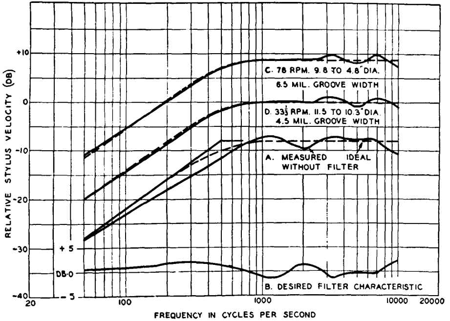
Fig. 5-31. Curves showing: A (cutter response without filter) B (desired filter characteristic) C (cutting characteristics with filter at 78 rpm) D (cutting characteristics at 33 1/3 rpm).
