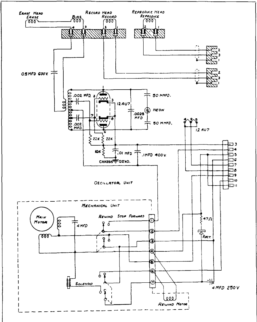
Fig. 12-36. Schematic of the Magnecorder PT63-A Oscillator Unit.
