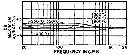
Fig. 20-12. Max. error in I.f. response resulting from use of 300-, 500-, and 800-cycle equalization for 250-1000 turnover points.
