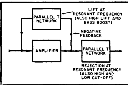
Fig. 16-19. Method of using parallel-T networks with an amplifier to give various frequency-response characteristics.
