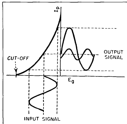
Fig. 28-1. Distortion in non-linear amplifier.
