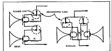
Fig. 22-18. The use of "grasshopper fuses" as a protection device. (Courtesy University)
