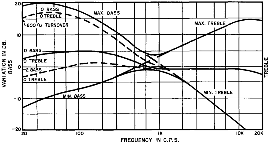
Fig. 26-7. Typical curves of the AE-2 preamp-equalizer.
