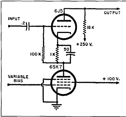
Fig. 19-43. The basic expander circuit, with typical circuit constants.
