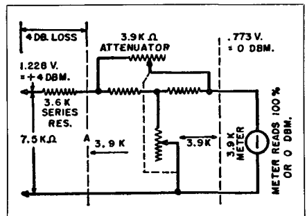
Fig. 8-10. Standard attenuating network for use with NARTB meter.
