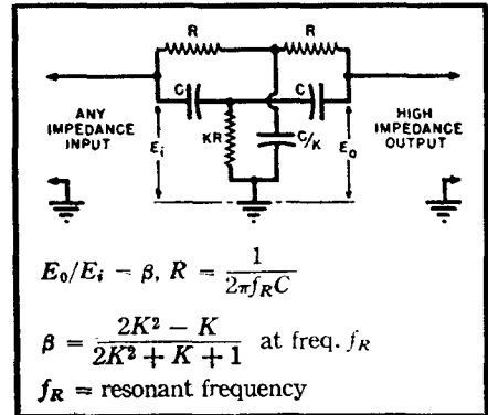
Fig. 16-20. Basic parallel—T R-C filter.
