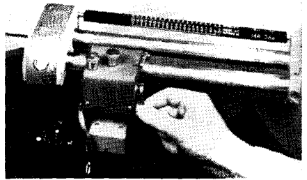
Fig. 5-24. Cutter-head is raised or lowered by this lever and permits gentle action.
