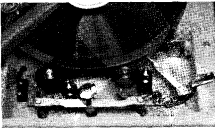
Fig. 5-19. Shows the position of the idlers with speed change knob "up" at 33 1/3 rpm.
