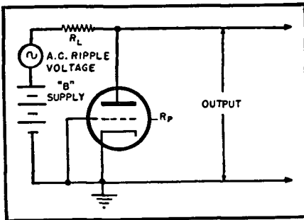
Fig. 28-27. Voltage divider effect attenuating plate supply ripple. The tube output is less than the "B" supply ripple by approximately the ratio of plate load resistance to plate impedance of the tube.
