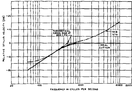
Fig. 5-27. NARTB Standard lateral recording characteristic and ideal cutter curve with crossover point at 500 cycles.
