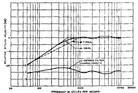
Fig. 5-28. Curves showing A (ideal cutter characteristic) B (typical response of MI-11850-C recording head) C (difference between A and B which gives the desired filter characteristic).
