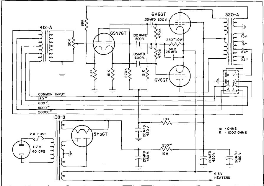
Fig. 25-15. Schematic of Langevin type 130A monitor amplifier.
