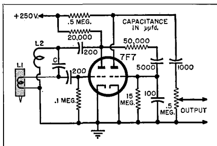
Fig. 9-13. Movement of pickup stylus amplitude-modulates an oscillating detector amplifier. Audio signal is obtained at output.
