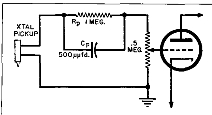
Fig. 4-14. Simple filter network that is often used for bass attenuation.
