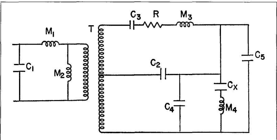
Fig. 9-27. Illustrating the action of the double torque-drive to actuate the crystal. C_1 is the compliance of the stylus; M_1 the mass of the stylus; M_2 is the mass of the pickup and tone-arm; T is the mechanical transformer; C_2 is the compliance of the top hinge at A and B in circuit (Fig. 9-25) which must bend before the force is transmitted to the crystal; C_3 is the compliance of the bottom hinge; R is the damping resistances to rotation of crystal and harness; M_3 is the effective mass of the crystal and drive mechanism for a rotating motion; C_X is the compliance of the crystal; C_4 is the compliance of the legs AF, AE, BC and BD for compressional motion; C_5 is the compliance of the legs HF, HC, GE and GD for compressional motion and M_4 is the effective mass of the crystal for the distorting motion.
