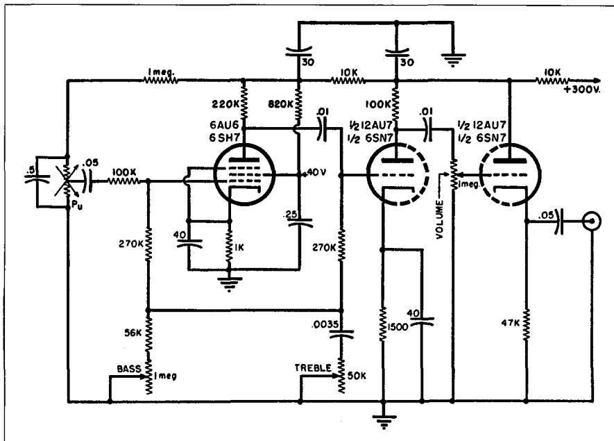
Fig. 9-11. The special preamplifier used with the strain-sensitive pickup. The cathode follower output permits the use of fairly long leads to a remote amplifier without excessive high frequency attenuation. High-impedance output may be taken from the plate of the first section of the dual triode if desired.
