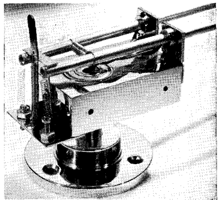
Fig. 10-12. Detailed construction of the Goodell Duplex reproducer arm.
