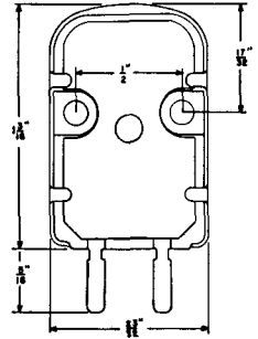
Fig. 9-36. Cut-away drawing shows the novel construction of the Model 12D cartridge.
