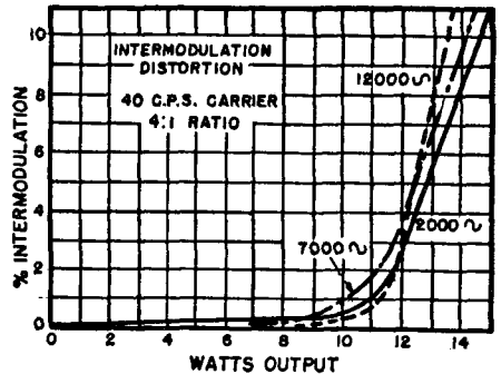
Fig. 21-5. Intermodulation distortion curves.
