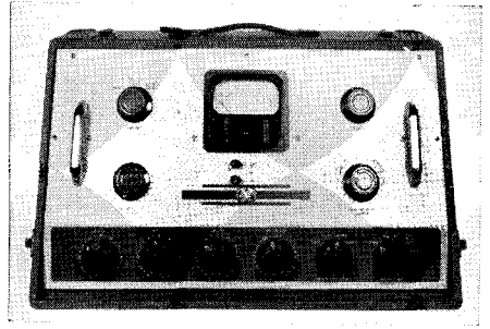
Fig. 26-31. The Presto 90-B portable recording console, described in the text. (Courtesy Presto)
