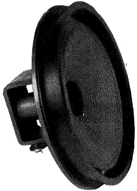
Fig. 15-17. RCA accordion cone, 7-inch permanent magnet speaker.
