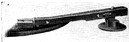
Fig. 10-13. The Audax Model L-6 tone arm and reproducer.
