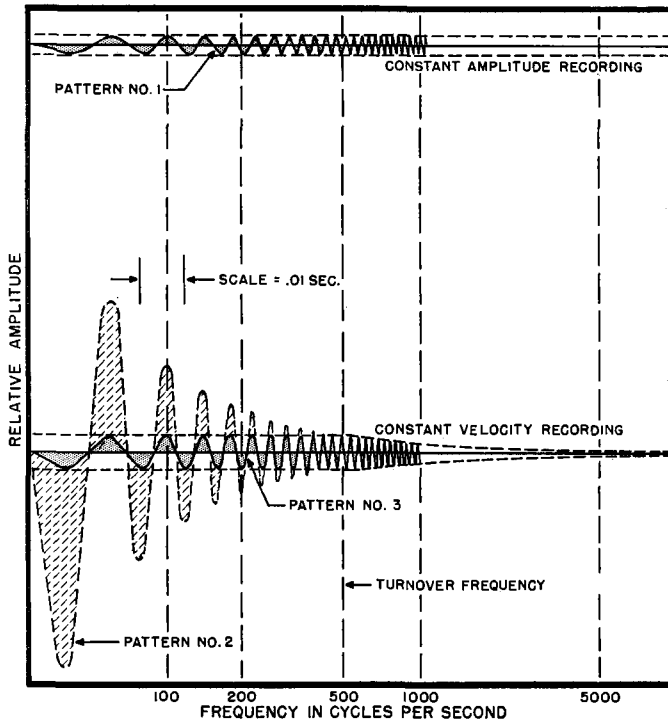
Fig. 4-21. Wave patterns for "constant amplitude" versus "constant velocity" recording.
