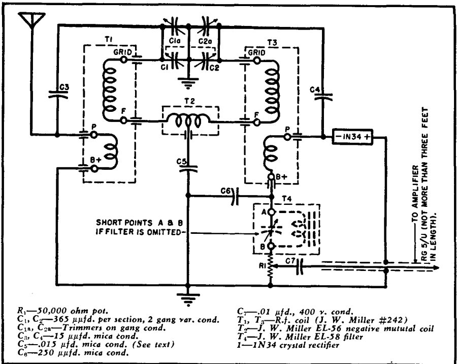
Fig. 24-1. Schematic diagram of a bandpass type tuner, using a crystal detector.
