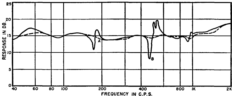
Fig. 15-34. Response frequency characteristics of a 15" loudspeaker mechanism mounted in the cabinet shown in Fig. 15-32. (A) Good response obtained by treating inside of cabinet with damping material. (B) Poor response when damping material is omitted.
