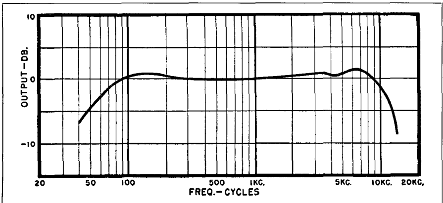
Fig. 3-17. Over-all frequency response of 35 mm. magnetic recording system.
