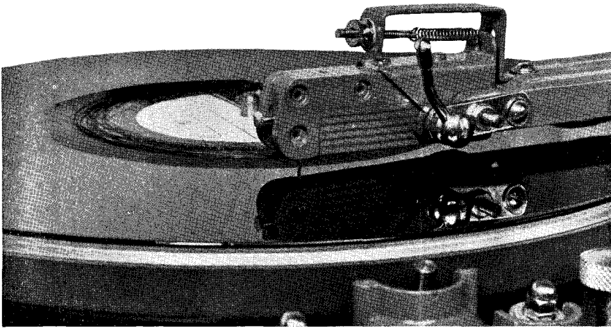
Fig. 4-22. The Brush RC-20 crystal cutter mounted correctly on a low plane and parallel to the record disc. (Courtesy, Radio & Television News)
