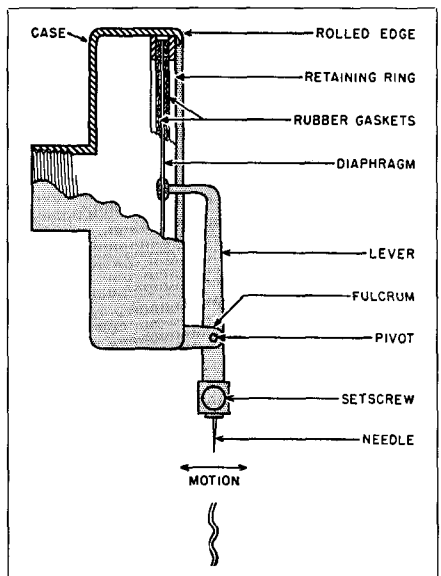
Fig. 2-7. Construction of an acoustical reproducer used with early phonographs.
