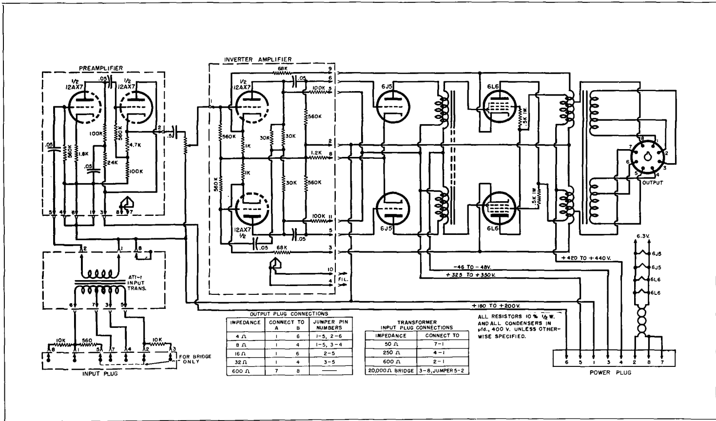
Fig. 26-19. Schematic of the McIntosh 50W-2 recording amplifier.
