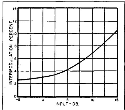
Fig. 3-18. Intermodulation distortion vs. recording level.
