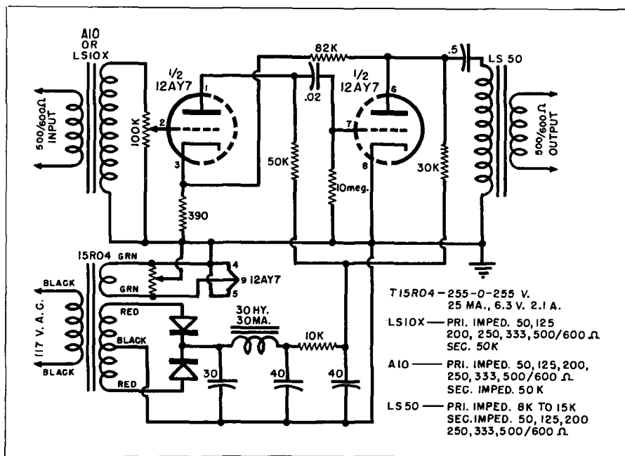
Fig. 26-9. Schematic of the line amplifier, using quality components for noise-free amplification.
