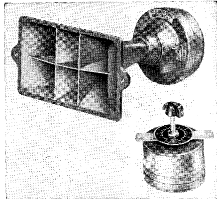
Fig. 15-43. Atlas Multi-cellular tweeter with high-frequency volume control. (Courtesy Atlas Sound)
