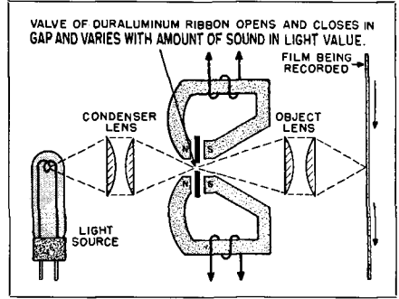
Fig. 3-5. The essential elements employed in variable density recording.
