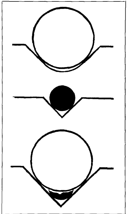
Fig. 7-22. Nearly all laterally cut records produced since 1900 can be played satisfactorily with a 2.5 mil stylus (top). Microgroove and 45 rpm records must be played with a stylus having a 1.0 mil tip (center). Standard depth records cut with V-groove ANM styli can be played back with either 1.0 or 2.5 mil styli (bottom).
