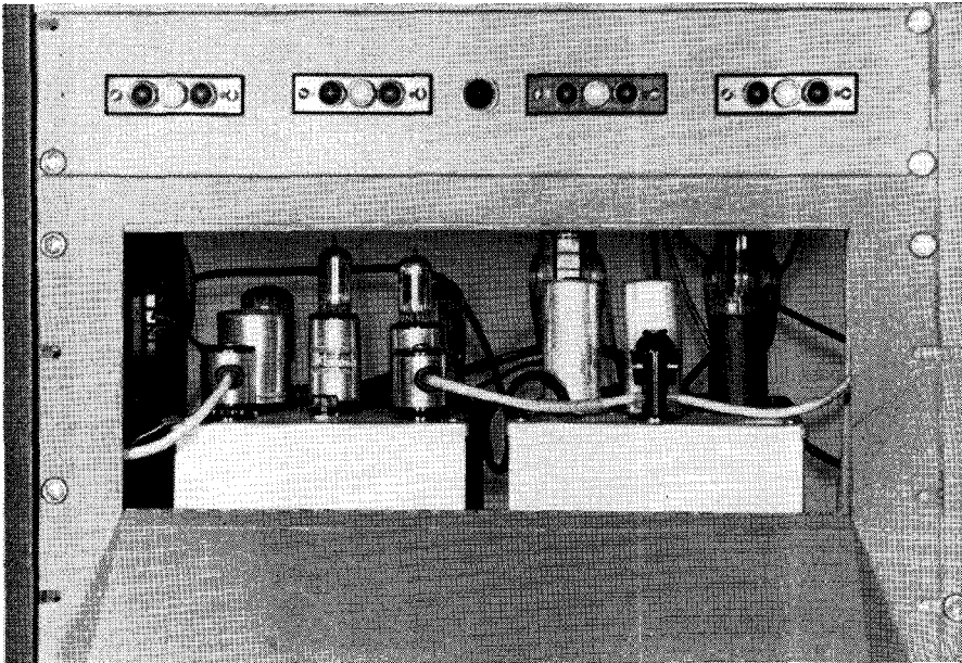
Fig. 26-20. The 50W-2 is mounted back of a hinged panel for easy mounting. (Courtesy RADIO & TELEVISION NEWS)
