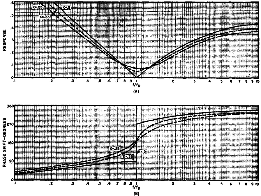
Fig. 16-15. (A) Amplitude response and (B) phase characteristics of parallel-T circuit shown in Fig. 16-20, for various values of the parameter K .
