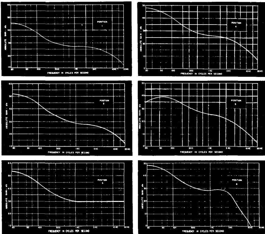
Fig. 17-31. Frequency response curves Model 132E, record compensator with Pickering Model 130H pre-amplifier equivalent. (Courtesy Pickering & Co.)
