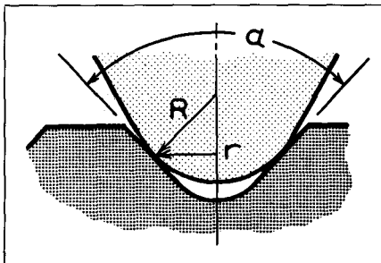
Fig. 7-25. Cross-sectional view of reproducing stylus in contact with record groove. (Courtesy, Columbia Records)
