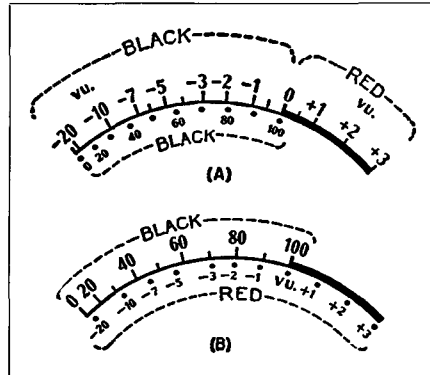
Fig. 8-9. (A) Standard VU type A scale stressing VU and (B) Standard VU scale type B stressing modulation.
