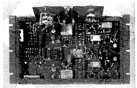
Fig. 25-17. Bottom view of the Presto 41-A peak limiting amplifier. (Courtesy Presto)
