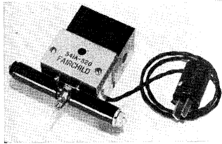
Fig. 5-39. The Fairchild 541 magnetic cutter head used with the 523 studio recorder.
