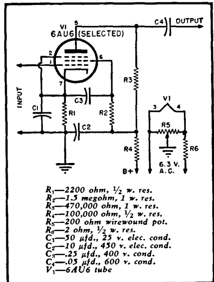
Fig. 28-31. Low-noise preamp using 6AU6.
