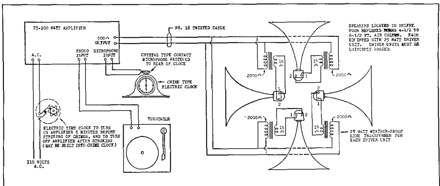
Fig. 22-15. A 75-100 watt church steeple installation. (Courtesy University)
