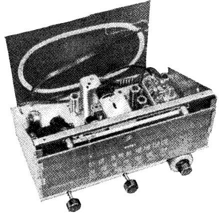
Fig. 24-6. The Espey model 512 FM-AM tuner chassis. (Courtesy Espey)
