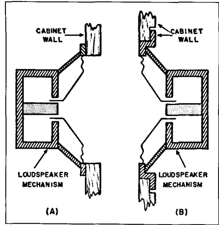
Fig. 15-35. Two different methods of mounting direct radiator loudspeaker mechanisms in wall of cabinet. (A) With mechanism mounted on back of cabinet wall. (B) Mechanism mounted flush with front surface of cabinet.
