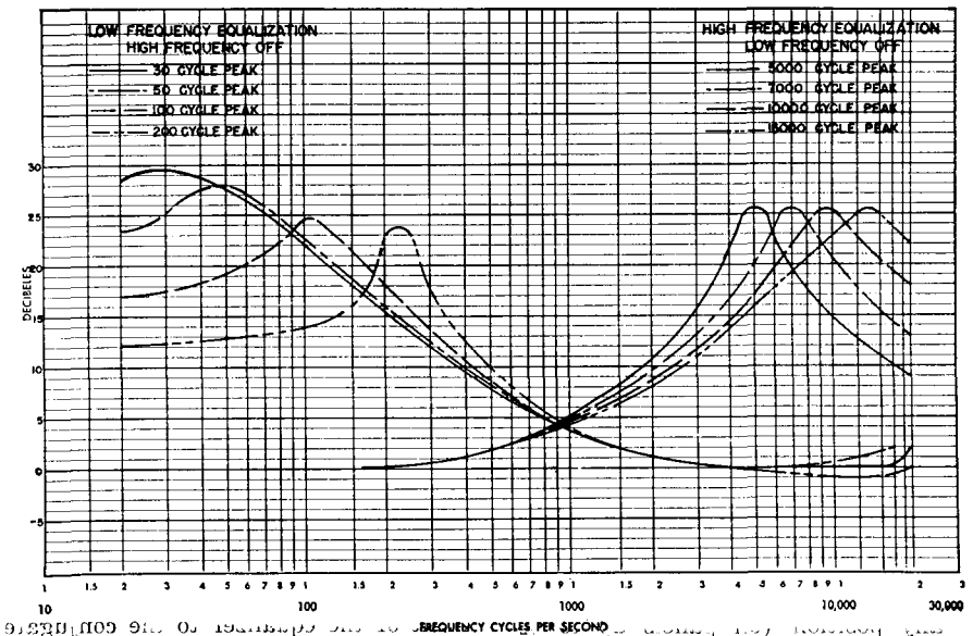
Fig. 17-36 Performance curves of the Collins 116F-1 program equalizer. (Joint)
