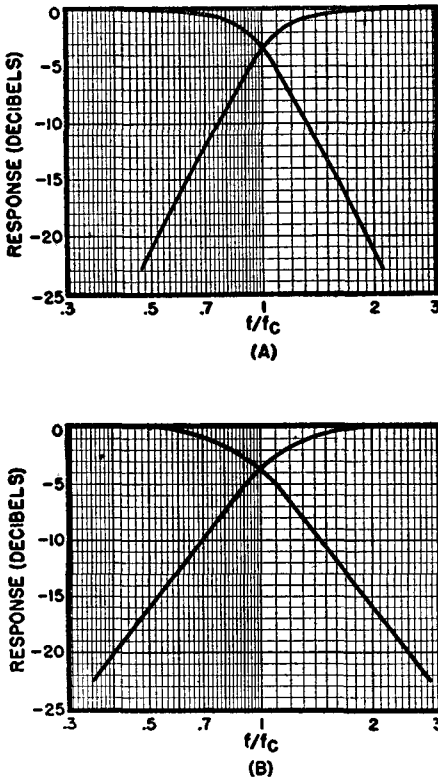
Fig. 16-16. Response curves of networks shown in Table 9. (A) is for the upper two networks, and (B) is for the lower two.
