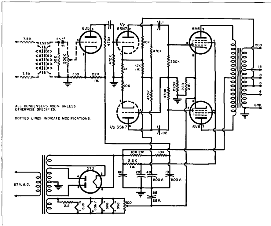
Fig. 26-2. Schematic diagram of the monitor amplifier using conventional circuits.
