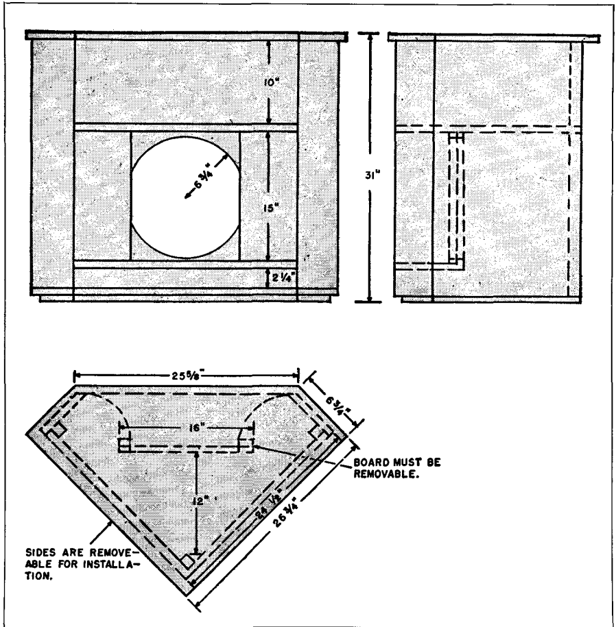
Fig. 15-6. Structural details of a corner cabinet for a single 15" loudspeaker.
