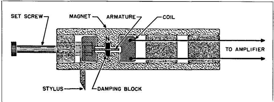
Fig. 4-12. Details of assembly and structure of Shure Model 96 magnetic cutter.
