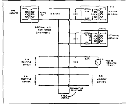
Fig. 26-17. Diagram of the bridging bus. Jacks are omitted for simplification.
