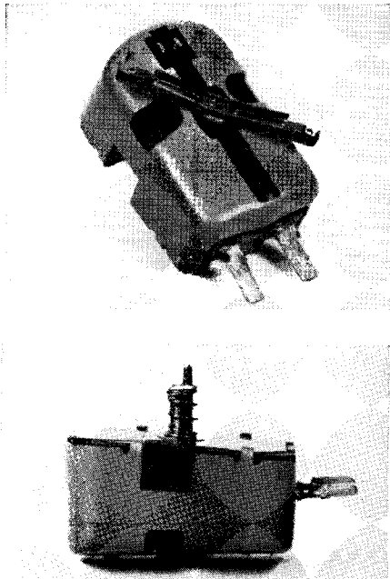
Fig. 9-34. Construction of the GE Model 12D triple play cartridge. (Courtesy, General Elect.)
