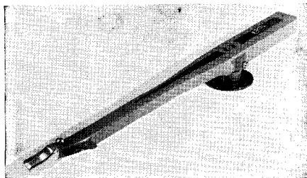
Fig. 10-14. The Audax studio arm with "tuned-ribbon" reproducer.
