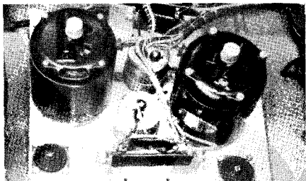
Fig. 5-16. Two hysteresis type motors rim-drive the turntable through rubber idler rollers.
