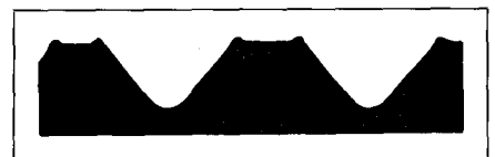
Fig. 7-26. Cross-section of groove showing how horns are thrown up on upper edges of groove walls. (Courtesy, Columbia Records)
