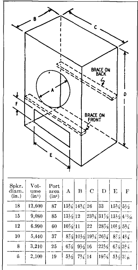
Fig. 15-9. Construction of a typical bass reflex speaker enclosure.
