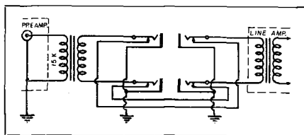
Fig. 26-10. Detailed schematic showing how double jacks connect between preamp and line amp.
