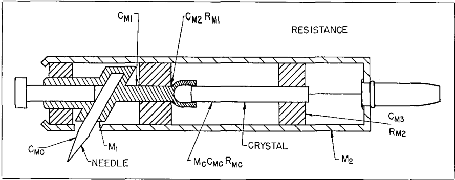
Fig. 9-26. Construction of the Bimorph type phono cartridge.
