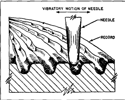
Fig. 9-1. Greatly enlarged cross-sectional view shows needle following record grooves.
