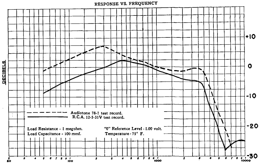
Fig. 9-33. Response curve of the ACD-1J cartridge.
