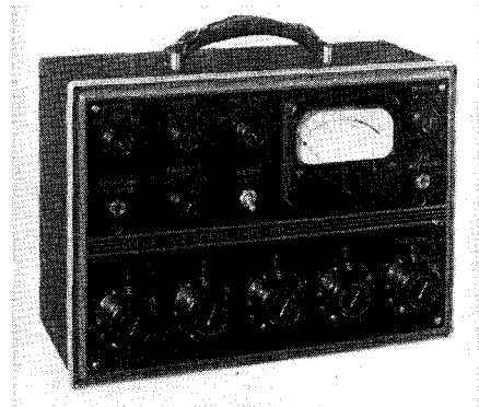
Fig. 25-6. Collins 12Z-2 remote amplifier. (Courtesy Collins Radio Co.)
