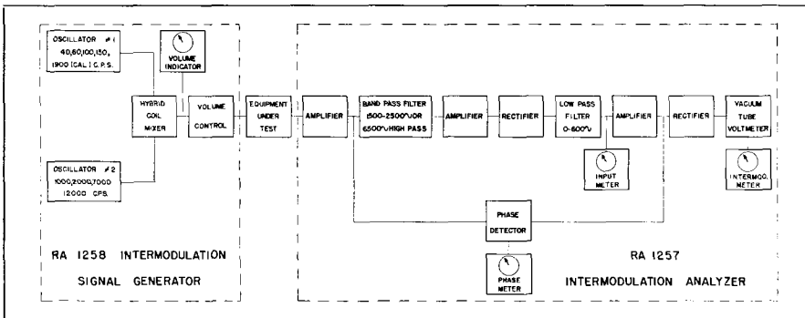
Fig. 28-8. Western Electric RA-1258 intermodulation signal generator (top), RA-1257 intermodulation analyzer (center), and block diagram of a complete setup for intermodulation measurements. (Courtesy Western Electric.)
