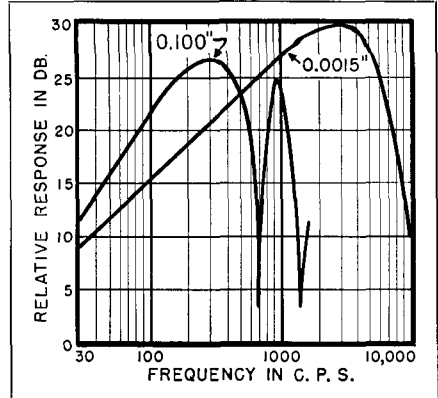
Fig. 11-13. Frequency vs. response curves show result when gap length is changed.
