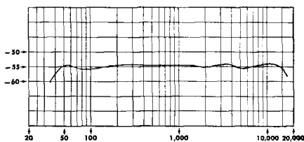
Fig. 14-38. Frequency response characteristics of the Electro-Voice model 655 dynamic microphone.
