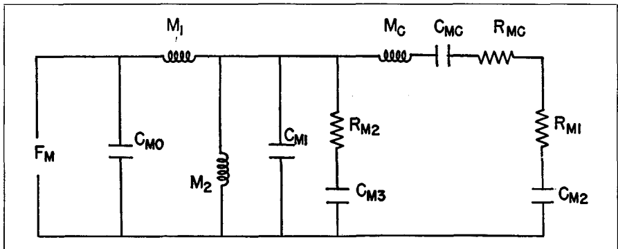
Fig. 9-23. Electrical circuit for a Bimorph phono cartridge.
