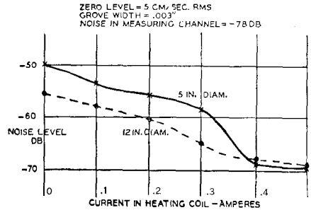
Fig. 7-29. Curve showing noise level in unmodulated groove vs. current in stylus heating coil. The noise is measured with a playback channel having uniform velocity response over a frequency band extending from 500 to 8000 cps.
