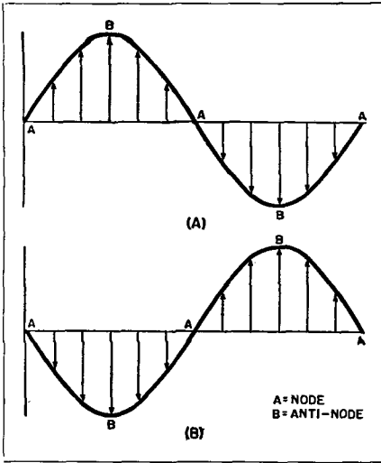
Fig. 1-5. Illustrates displacement of waves.
