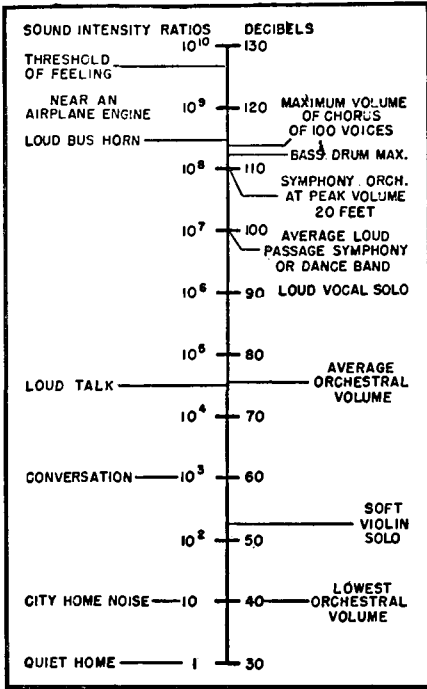
Fig. 23-13. Loudness levels of everyday sounds shown in db and in sound intensity ratios.
