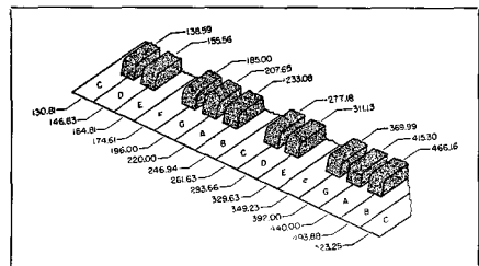
Fig. 1-2. Diagram illustrates keys of a piano keyboard and shows tempered scale for one octave on each side of middle C.
