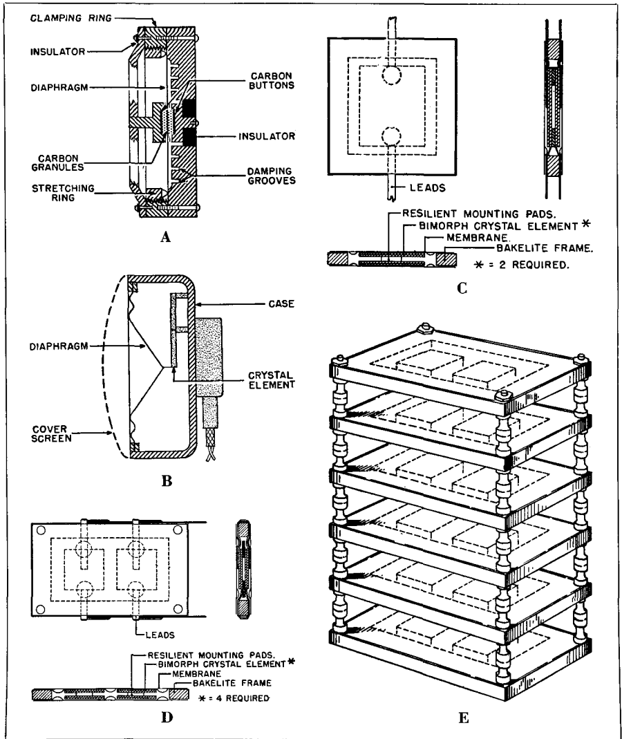
Fig. 14-4. (A) Double button carbon, (B) crystal diaphragm, (C) single crystal element, (D) multiple crystal element and (E) six element sound cell construction.
