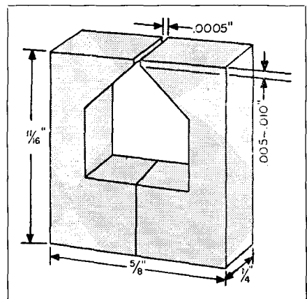
Fig. 12-3. Mechanical details show construction of a record-playback head.
