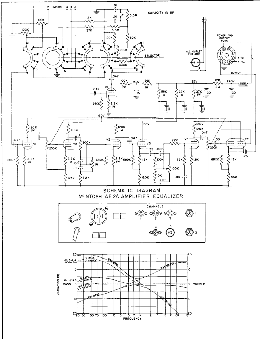
Fig. 20-8. Schematic diagram of the McIntosh AE-2A amplifier equalizer.
