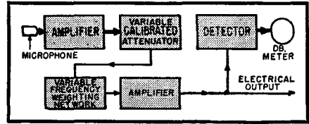
Fig. 23-7. Basic block diagram of a sound-level meter.
