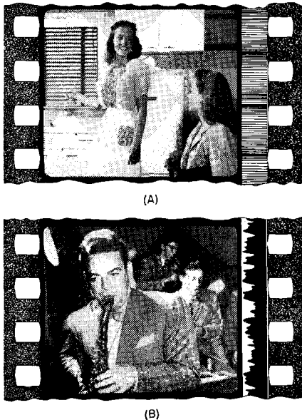
Fig. 3-4. (A) Variable density sound track on 35 mm. movie film. (B) Variable area sound track as it appears on a single frame.
