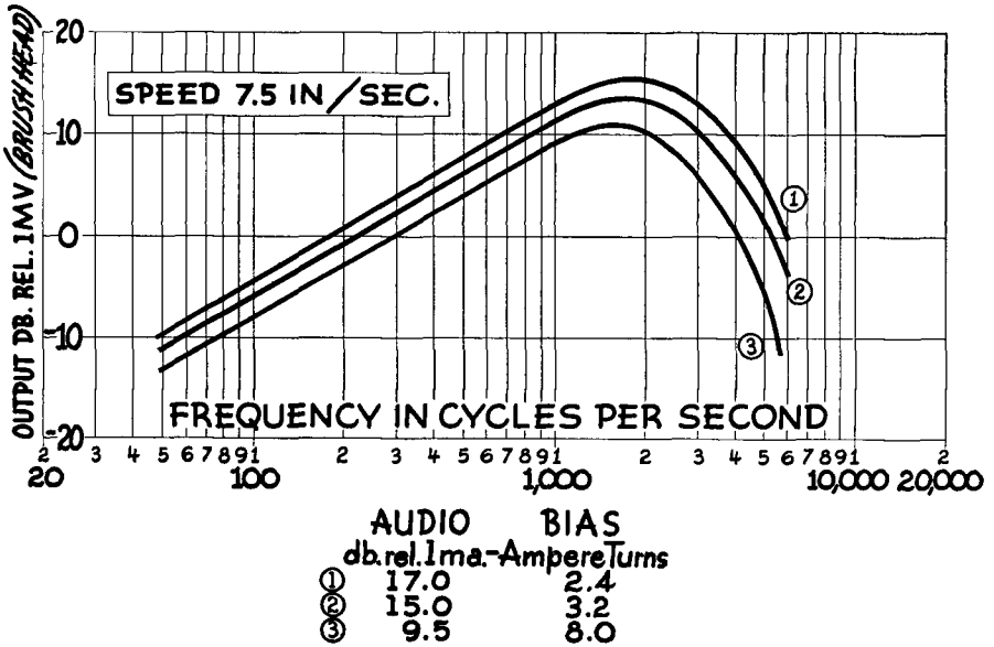
Fig. 11-17. Effect of Bias on Frequency Response. "Scotch" Sound Recording Tape No. 111.
