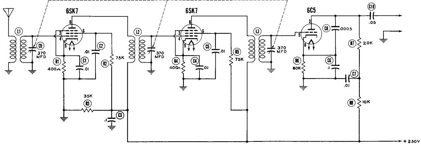
Fig. 24-2. Schematic of a conventional TRF (Tuned radio frequency) Tuner.
