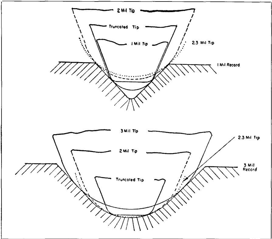
Fig. 9-28. Showing the comparative fits of 3-mil, 2-mil and 2.3-mil truncated type styli in 1-mil and 3-mil record grooves. (Courtesy, Electro-Voice)
