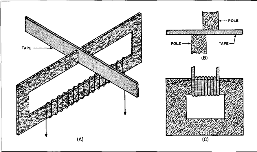
Fig. 11-11. (A) Record-reproduce head for transverse recording on tape. (B) Offset thick pole pieces used to improve characteristics of head shown in (A). (C) The closed type record-reproduce wire head used in some types of magnetic recorders.
