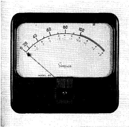
Fig. 8-8. Standard VU meter, Simpson 49, with B scale. (Courtesy, Simpson Elect.)
