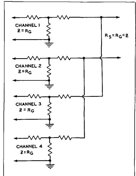
Fig. 18-8. Four-channel parallel-series mixer whose loss is 6 db and whose impedance ratio is unity.
