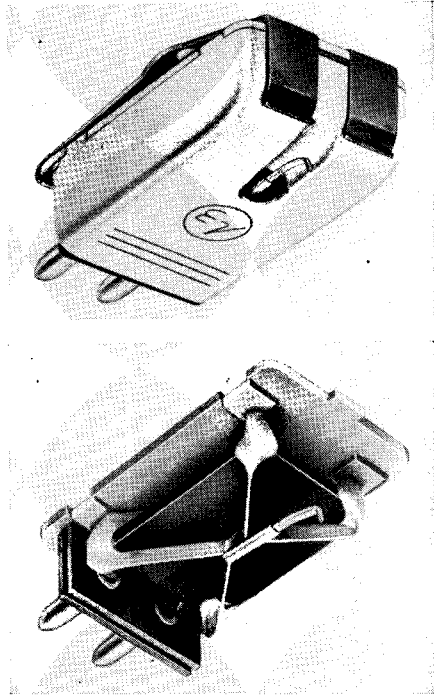
Fig. 9-24. (A) The Electro-Voice series 12 phono cartridge. (B) View of torque-drive cartridge with case removed, showing position of the crystal and its harness.
