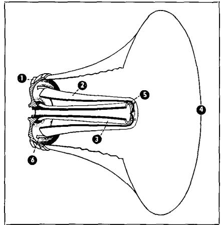
Fig. 22-22. The Racon exponential re-entrant trumpet (1) cast aluminum back (2) non-resonant exponential flared reflector (3) non-resonant exponential flared cast aluminum tone arm (4) exponential flared heavy spun aluminum bell (5) precision machined spacers maintain correct distance between tone arm and reflector (6) integrally cast bosses to provide reflector concentricity and spacing between reflector and back casting. (Courtesy Racon)
