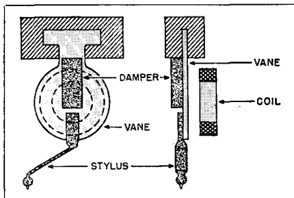
Fig. 9-12. Moving vane structure of Zenith "Cobra" pickup.
