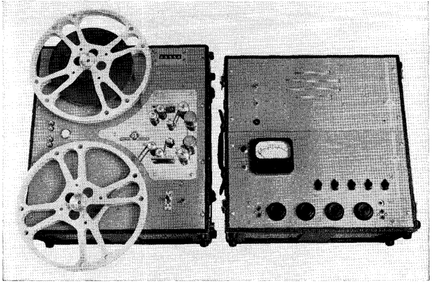
Fig. 13-11. The Stancil-Hoffman SR-Synchronous film recorder. (Courtesy Stancil-Hoffman)
