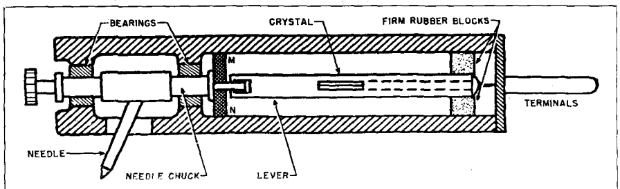
Fig. 9-8. Motions of the needle chuck are transmitted to the crystal via lever action in this Shure-designed crystal cartridge.
