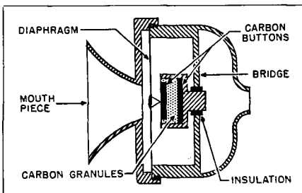
Fig. 14-1. Single button carbon microphone.
