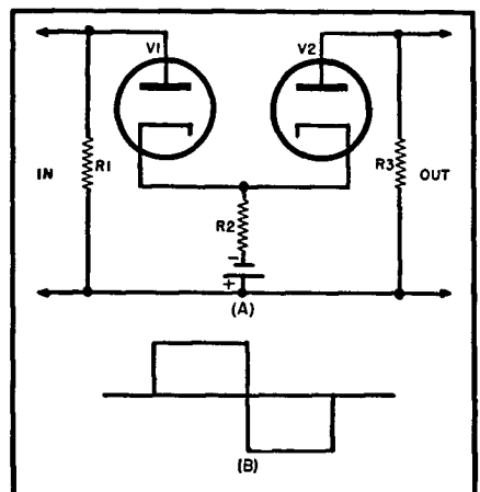
Fig. 28-20. Clipper circuit. See text for values of components.
