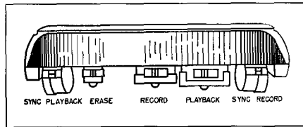
Fig. 13-13. Details of the Rangertone 5 head assembly. (Courtesy Rangertone)
