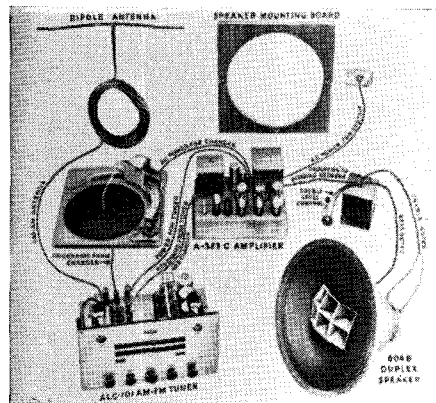
Fig. 21-11. Necessary quality components for a complete home music system. (Courtesy Altec Lansing)
