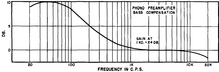
Fig. 24-12. Phono preamplifier characteristics.
