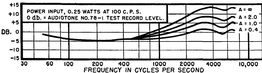
Fig. 4-16. Effect of resistance across cutter in pentode circuits. The ratio of the parallel resistance to the cutter impedance is represented by A.
